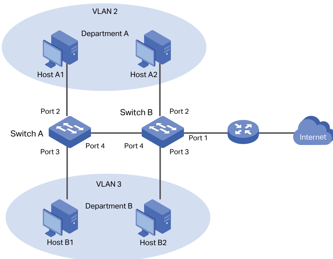
Figure 3-1 Network Topology
